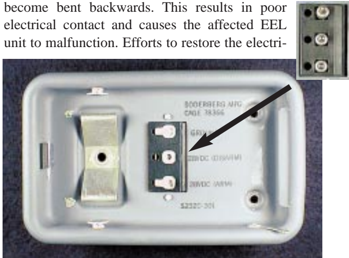
The original leaf-type contactors on the light base have been replaced by rugged plunger-type contactors.
